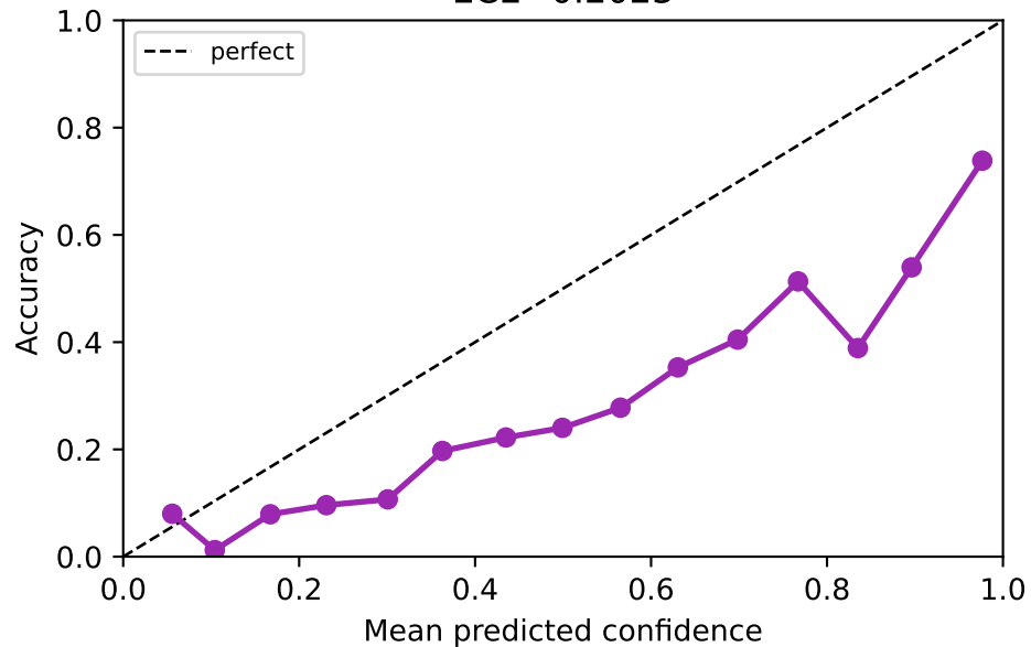
After temperature scaling ECE=0.2023
