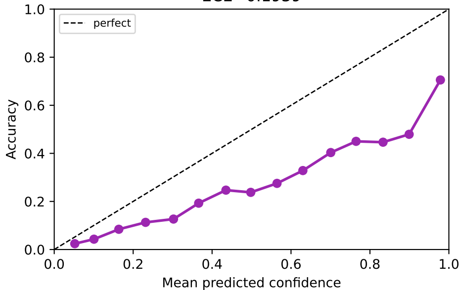
Before temperature scaling ECE=0.1939
